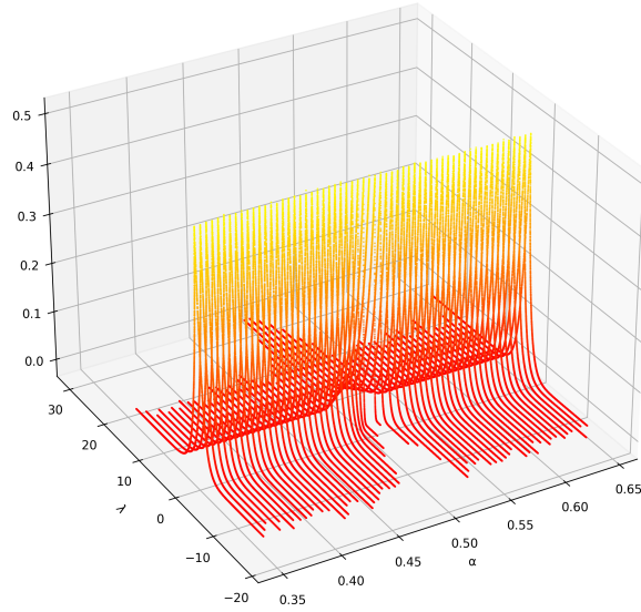
FIGURE 4. A discrete approximation of the probability density function associated to \widehat{\mathcal{S}}_{\pi, \Psi}(X_1, X_2, T, \rho_{\pi}) where L(s, \pi) = \zeta(s) , X_1 = T^{\frac{1}{2}} and X_2 = T^{\alpha_2} with \alpha_2 varying between (0.35, 0.65) in a discrete equi-spaced manner.
